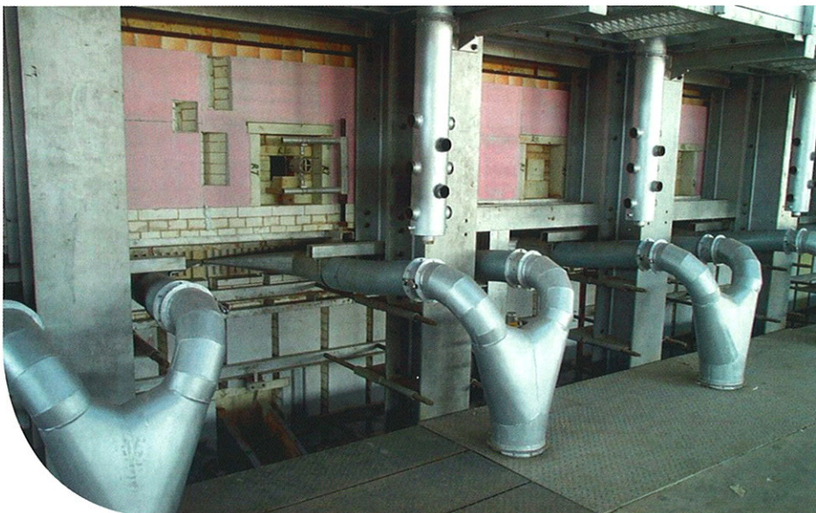
Furnace cooling network
